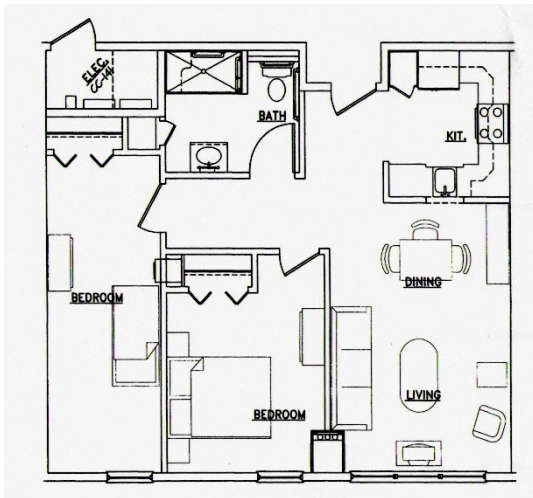
Typical Two Bedroom Design (775 SqFt.)
