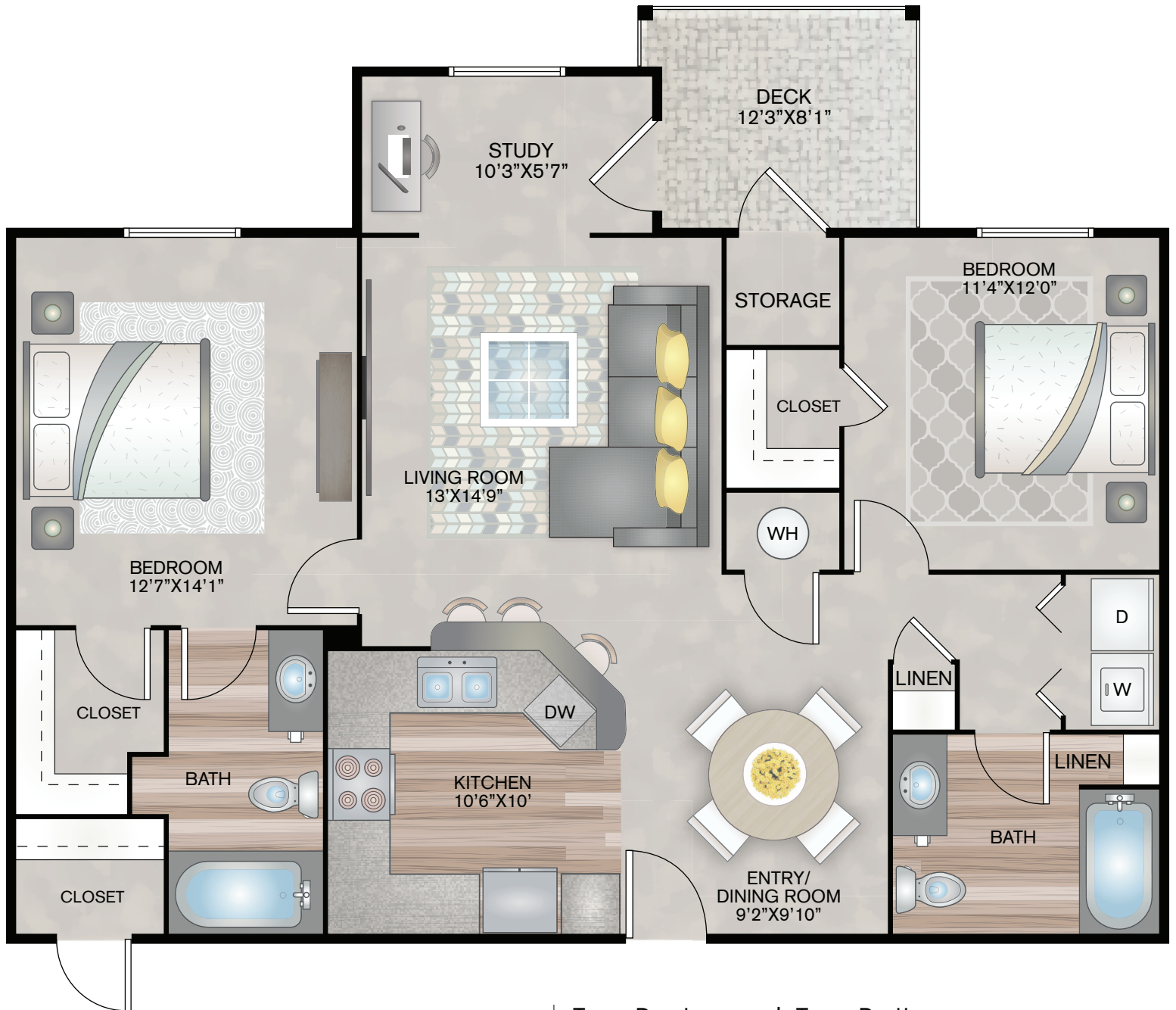
ALL AMERICAN | Two Bedroom | Two Bath 1,180 Sq Ft
